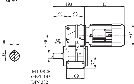
GFA/GFH/GFV47
