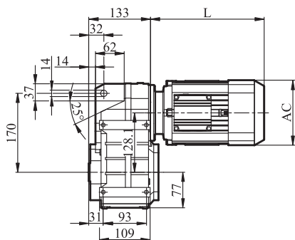
GFA/GFH/GFV47
